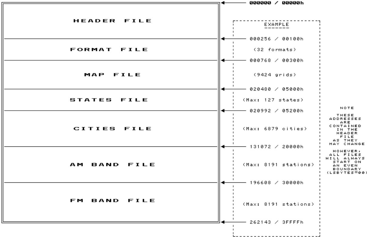
Figure 48 - 256 kilobyte ROM structure
