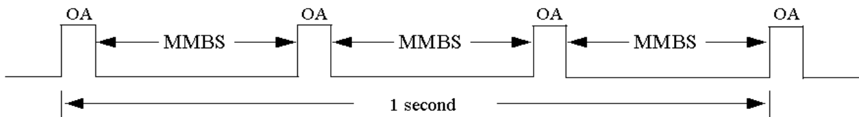
Figure P.3: Typical multiplex coding
