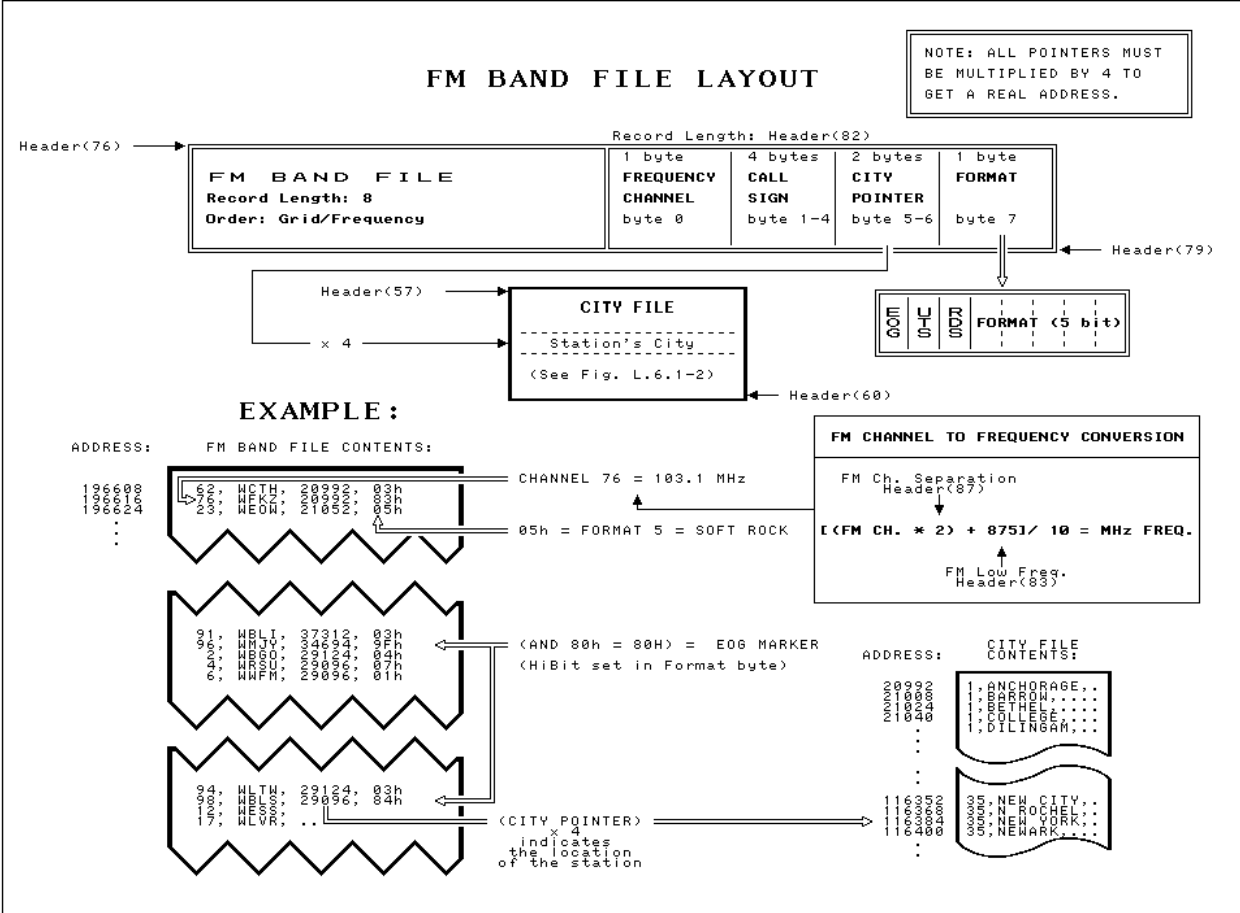
Figure R.8 - FM Band File layout
